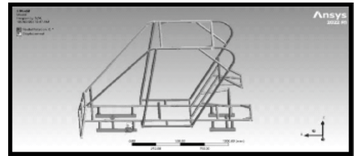
Fig. 33: Nodal force for Hard point
