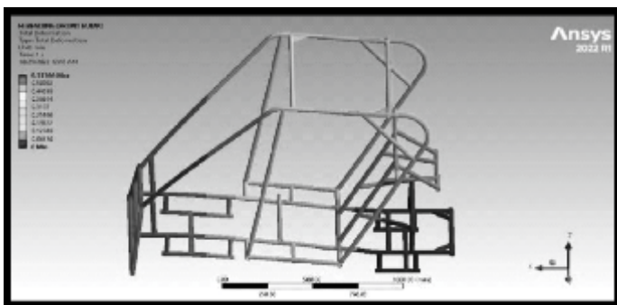
Fig. 24: Front bump Deformation
