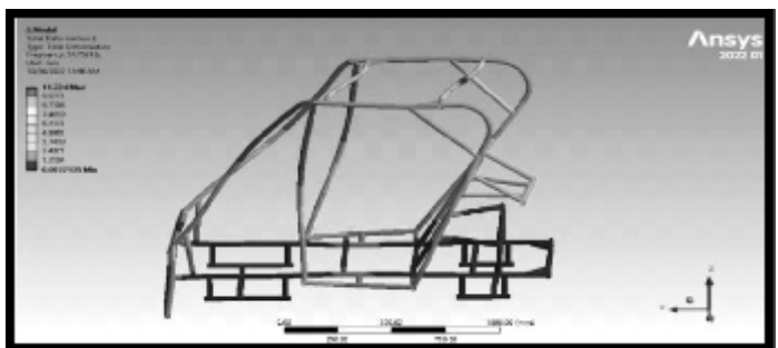
Fig. 35: Mode shape 2
