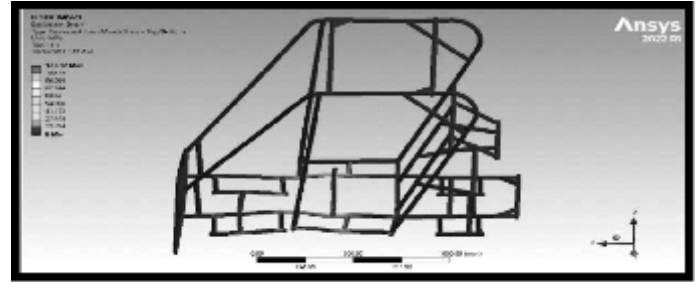
Fig. 11: Side Impact Stress
