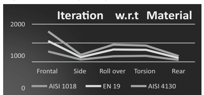
Fig. 5: Iteration stress results w.r.t. Material
