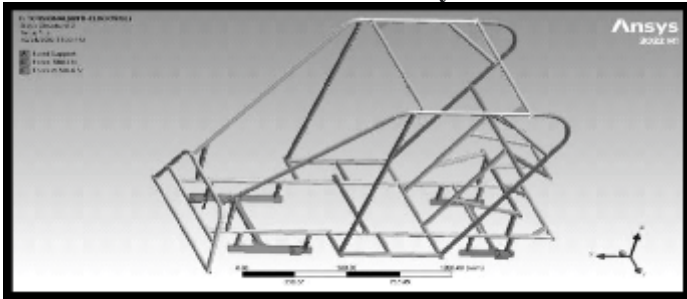
Fig. 31: Nodal force for Torsional(anti-clockwise)
