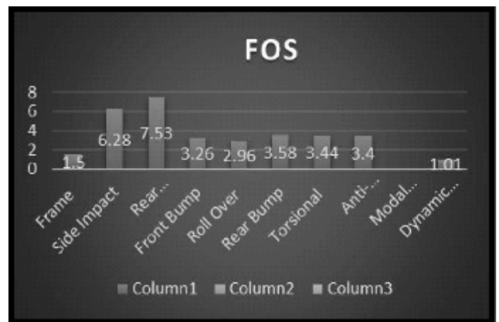
Fig. 40: Factor of safety
