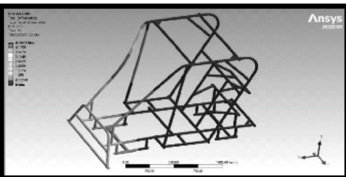
Fig.18: Rollover Deformation
