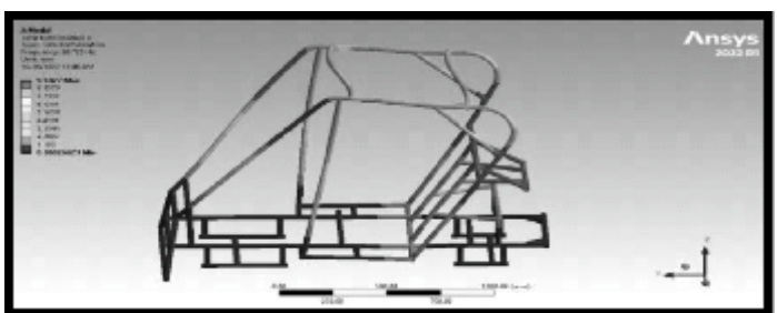
Fig. 36: Mode shape 3
